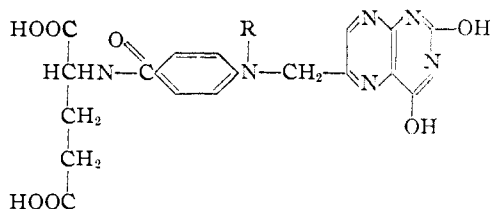
I, R = -N=O II, R = H
